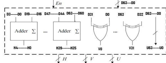
Fig.3 64-bit DMC encoder structure using multi bit adders and XOR gates
