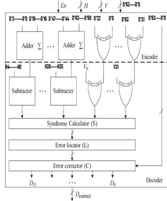
Fig.3 64-bit DMC encoder structure using multi bit adders and XOR gates
