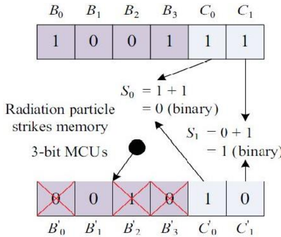
Fig .5 limits of binary error detection in simple binary operations
