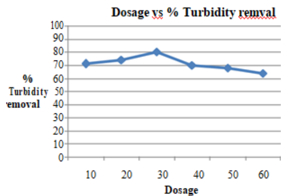
Chart 8: Dosage vs % Turbidity removal (Alum coagulant)
