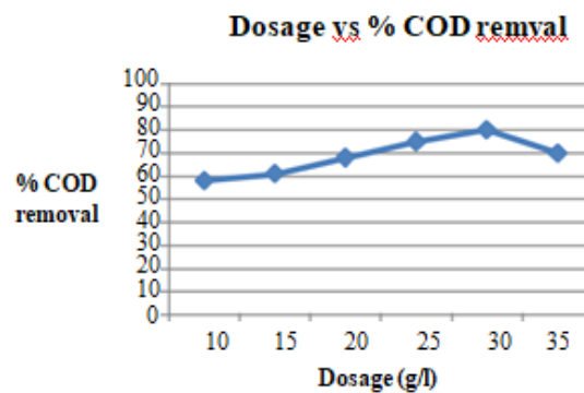
Chart 5: Dosage vs % COD removal (CaOH Coagulant)
