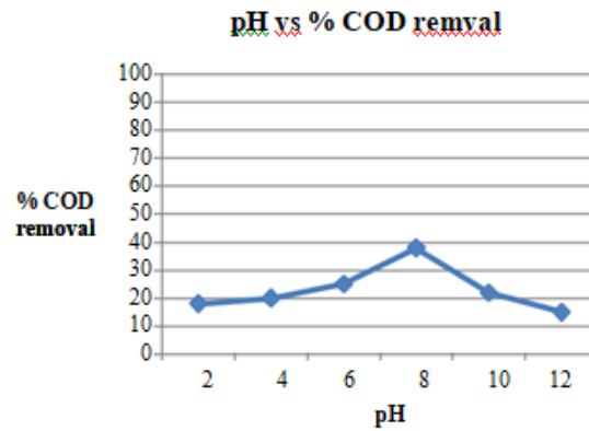
Chart 3: pH vs % COD removal (Alum coagulant)
