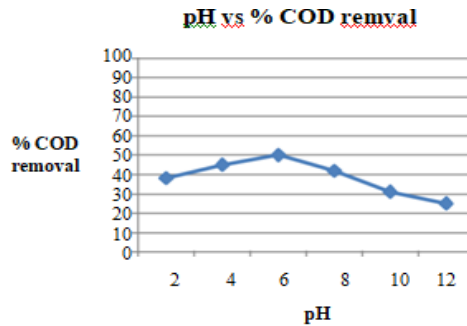
Chart 1: pH vs % COD removal (CaOH coagulant)
