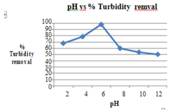
Chart 4: pH vs % Turbidity removal (Alumcoagulant)
