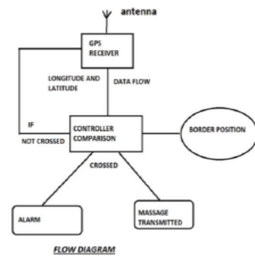
Fig.2. Block diagram
