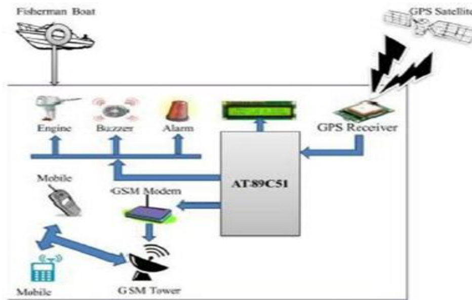
Fig.3. Microcontroller design
